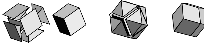
Figure 17: Constructing the rhombic dodecahedron
