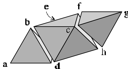
Figure 14: A subdivided parallelepiped
