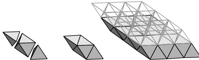
Figure 5: Slicing the packing through the plane of contact
