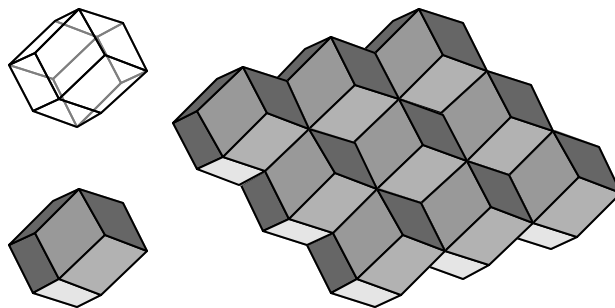
Figure 16: The rhombic dodecahedron and its packing
