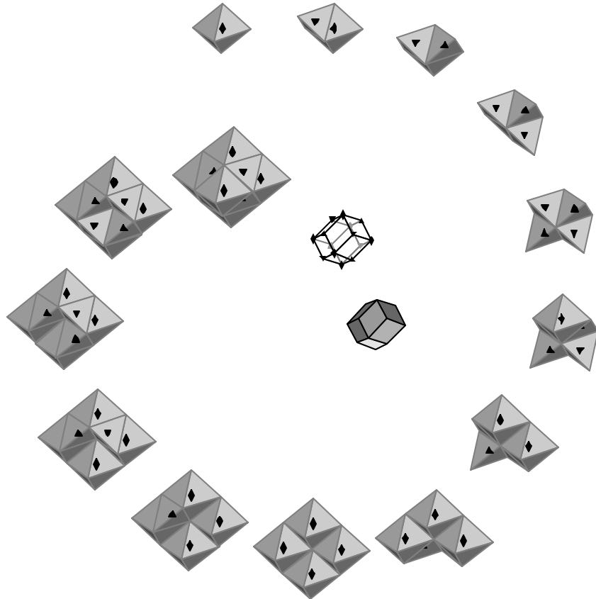
Figure 15: A vertex of the tetrahedral-octahedral space filler
