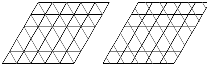
Figure 2: The triangle grid and the 3.6.3.6 Archimedean tiling
