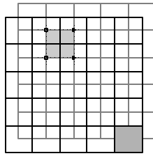
Figure 10: The square tiling is a self-dual
