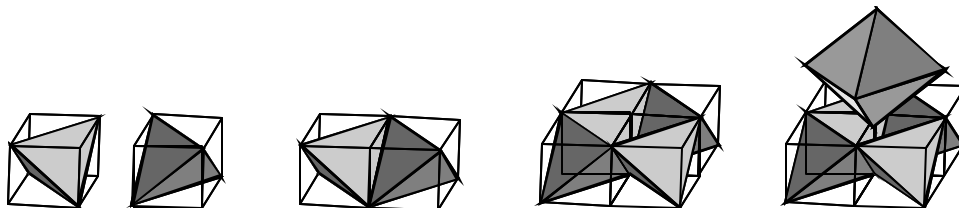
Figure 7: Assembling the tetrahedral-octahedral packing
