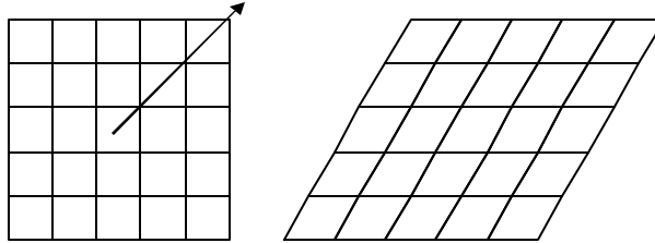
Figure 1: From the square tiling to the rhombic tiling
