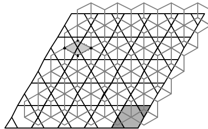
Figure 12: Dual of the 3.6.3.6 Archimedean tiling.
