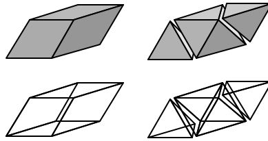
Figure 4: From a single parallelepiped to two tetrahedra and one octahedron
