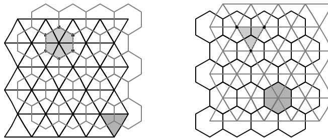
Figure 11: Triangular and hexagonal tilings are dual
