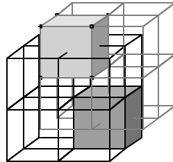
Figure 13: The cubic packing is self-dual
