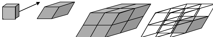
Figure 3: From the cube to the parallelepiped packing
