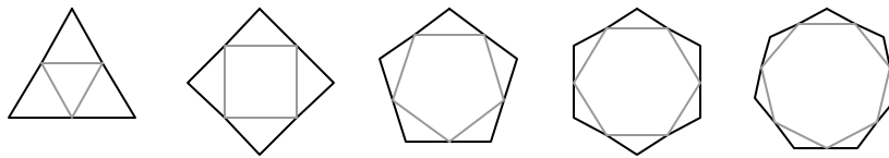
Figure 8: Polygons and their duals
